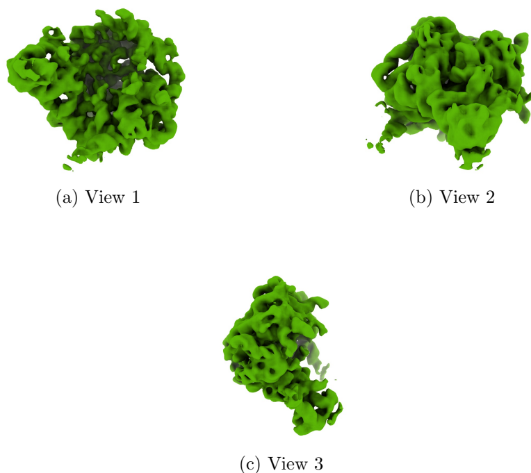
Figure 4: Isosurface at threshold=5.400000. Views generated by ChimeraX at a the following X, Y, Z angles: View 1 (0, -90, -90), View 2 (-90, 0, -90), View 3 (0, 0, 0).
