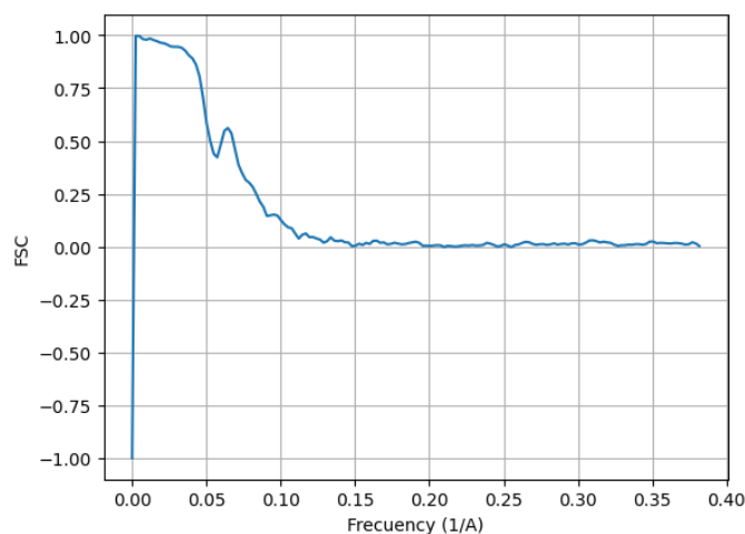
Figure 22: FSC and resolution estimated by a permutation test.
