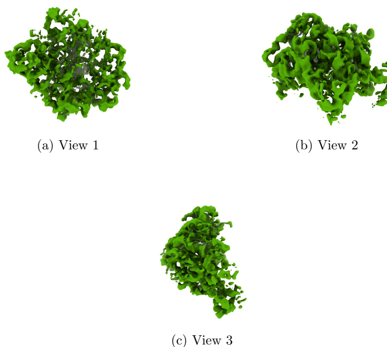
Figure 4: Isosurface at threshold=9.000000. Views generated by ChimeraX at a the following X, Y, Z angles: View 1 (0, -90, -90), View 2 (-90, 0, -90), View 3 (0, 0, 0).
