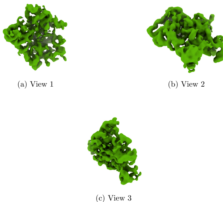
Figure 4: Isosurface at threshold=6.600000. Views generated by ChimeraX at a the following X, Y, Z angles: View 1 (0, -90, -90), View 2 (-90, 0, -90), View 3 (0, 0, 0).
