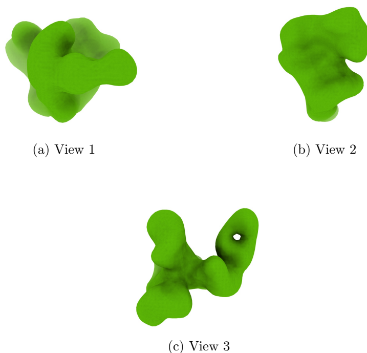
Figure 4: Isosurface at threshold=0.154100. Views generated by ChimeraX at a the following X, Y, Z angles: View 1 (0, -90, -90), View 2 (-90, 0, -90), View 3 (0, 0, 0).
