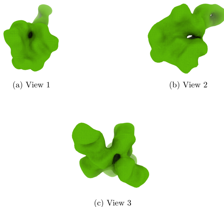
Figure 4: Isosurface at threshold=0.195500. Views generated by ChimeraX at a the following X, Y, Z angles: View 1 (0, -90, -90), View 2 (-90, 0, -90), View 3 (0, 0, 0).
