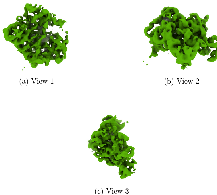
Figure 4: Isosurface at threshold=6.900000. Views generated by ChimeraX at a the following X, Y, Z angles: View 1 (0, -90, -90), View 2 (-90, 0, -90), View 3 (0, 0, 0).
