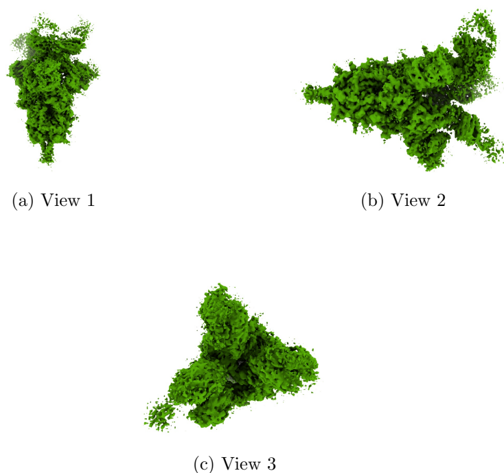
Figure 4: Isosurface at threshold=0.012600. Views generated by ChimeraX at a the following X, Y, Z angles: View 1 (0, -90, -90), View 2 (-90, 0, -90), View 3 (0, 0, 0).
