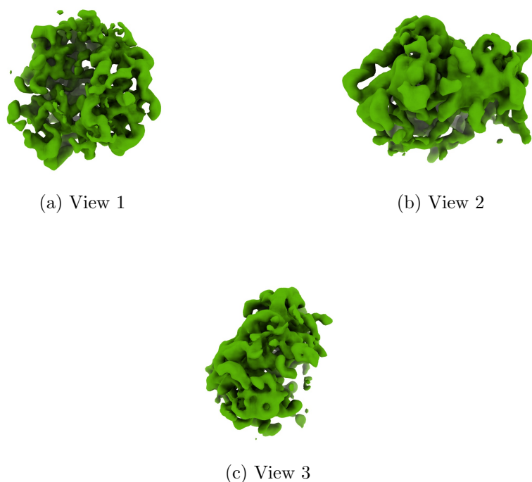
Figure 4: Isosurface at threshold=6.300000. Views generated by ChimeraX at a the following X, Y, Z angles: View 1 (0, -90, -90), View 2 (-90, 0, -90), View 3 (0, 0, 0).
