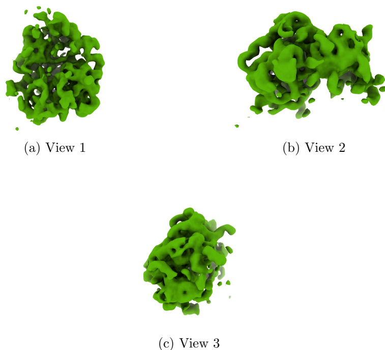
Figure 4: Isosurface at threshold=6.070000. Views generated by ChimeraX at a the following X, Y, Z angles: View 1 (0, -90, -90), View 2 (-90, 0, -90), View 3 (0, 0, 0).
