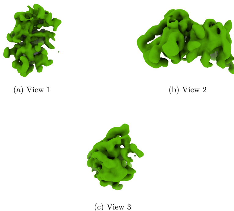
Figure 4: Isosurface at threshold=4.430000. Views generated by ChimeraX at a the following X, Y, Z angles: View 1 (0, -90, -90), View 2 (-90, 0, -90), View 3 (0, 0, 0).
