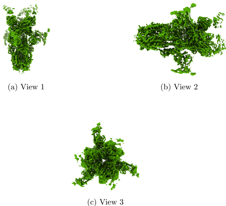
Figure 4: Isosurface at threshold=0.658000. Views generated by ChimeraX at a the following X, Y, Z angles: View 1 (0, -90, -90), View 2 (-90, 0, -90), View 3 (0, 0, 0).
