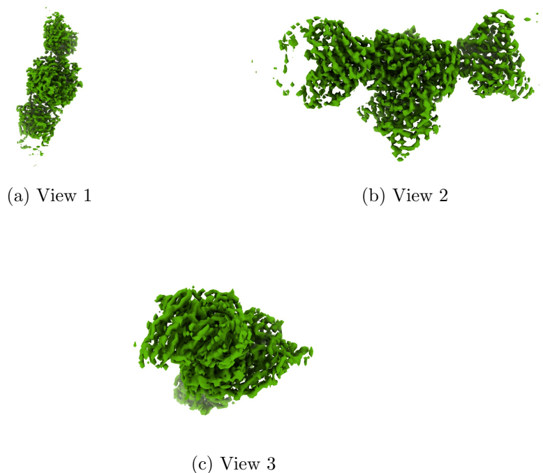
Figure 4: Isosurface at threshold=0.620000. Views generated by ChimeraX at a the following X, Y, Z angles: View 1 (0, -90, -90), View 2 (-90, 0, -90), View 3 (0, 0, 0).
