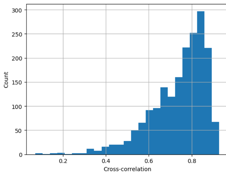
Figure 13: Histogram of the cross-correlation between the map and model evaluated for all residues.
