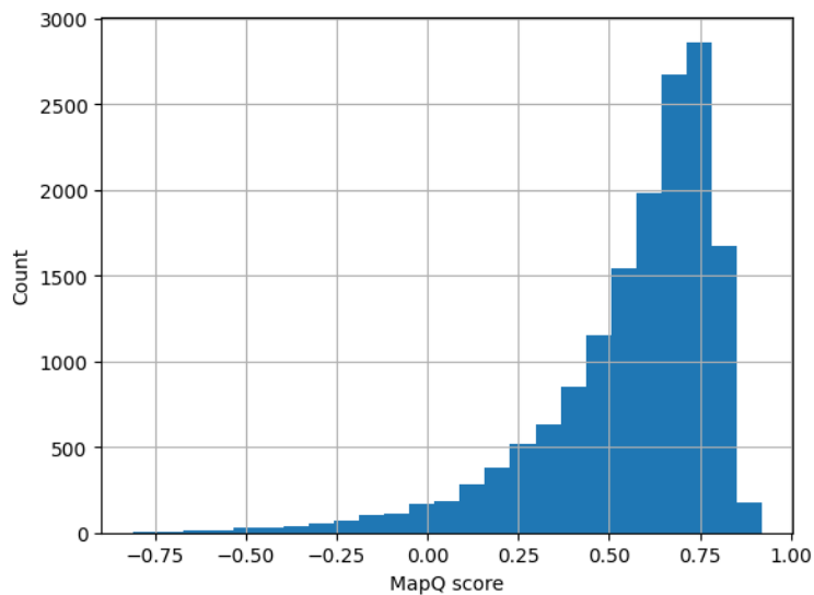
Figure 16: Histogram of the per-atom Q-score.
