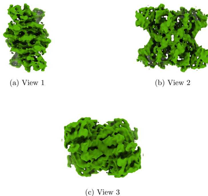
Figure 4: Isosurface at threshold=0.005950. Views generated by ChimeraX at a the following X, Y, Z angles: View 1 (0, -90, -90), View 2 (-90, 0, -90), View 3 (0, 0, 0).
