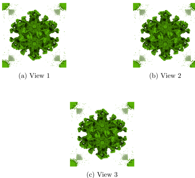
Figure 4: Isosurface at threshold=0.750000. Views generated by ChimeraX at the following X, Y, Z angles: View 1 (0, -90, -90), View 2 (-90, 0, -90), View 3 (0, 0, 0).
