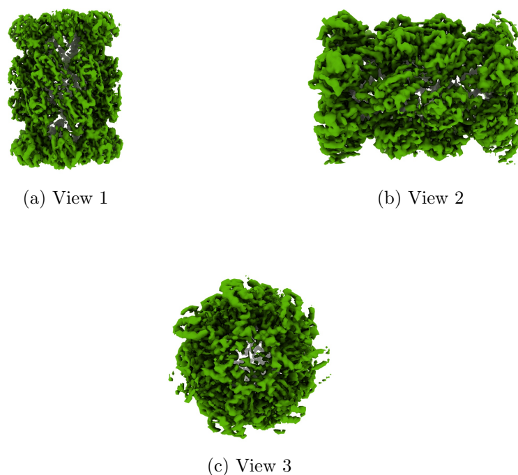
Figure 4: Isosurface at threshold=0.857000. Views generated by ChimeraX at a the following X, Y, Z angles: View 1 (0, -90, -90), View 2 (-90, 0, -90), View 3 (0, 0, 0).
