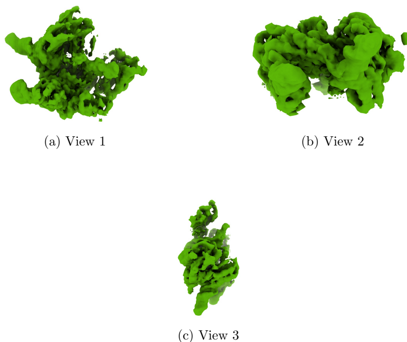
Figure 4: Isosurface at threshold=0.139000. Views generated by ChimeraX at a the following X, Y, Z angles: View 1 (0, -90, -90), View 2 (-90, 0, -90), View 3 (0, 0, 0).
