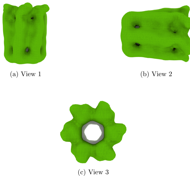
Figure 4: Isosurface at threshold=0.018061. Views generated by ChimeraX at a the following X, Y, Z angles: View 1 (0, -90, -90), View 2 (-90, 0, -90), View 3 (0, 0, 0).
