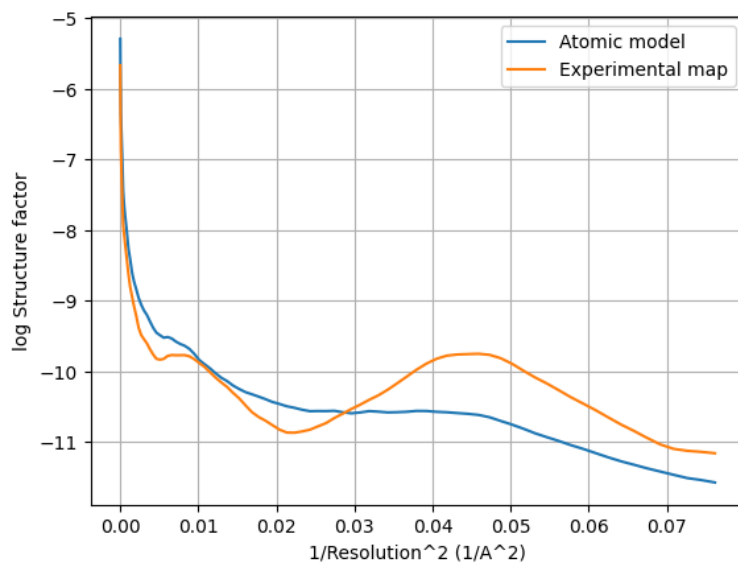
Figure 15: Guinier plot of the atom model and experimental map. The X-axis is the square of the inverse of the resolution in Å.
