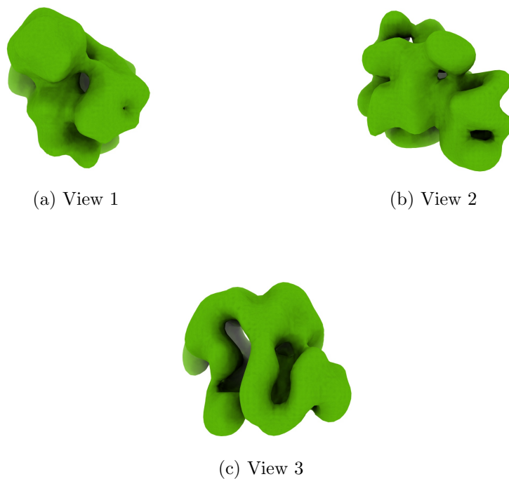
Figure 4: Isosurface at threshold=4.680000. Views generated by ChimeraX at a the following X, Y, Z angles: View 1 (0, -90, -90), View 2 (-90, 0, -90), View 3 (0, 0, 0).
