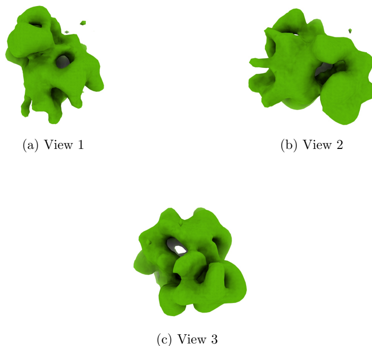
Figure 4: Isosurface at threshold=0.038500. Views generated by ChimeraX at a the following X, Y, Z angles: View 1 (0, -90, -90), View 2 (-90, 0, -90), View 3 (0, 0, 0).
