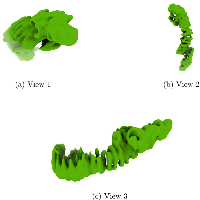
Figure 4: Isosurface at threshold=0.011900. Views generated by ChimeraX at a the following X, Y, Z angles: View 1 (0, -90, -90), View 2 (-90, 0, -90), View 3 (0, 0, 0).
