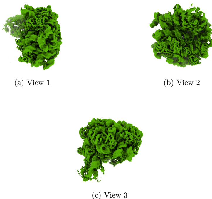
Figure 4: Isosurface at threshold=0.008270. Views generated by ChimeraX at the following X, Y, Z angles: View 1 (0, -90, -90), View 2 (-90, 0, -90), View 3 (0, 0, 0).
