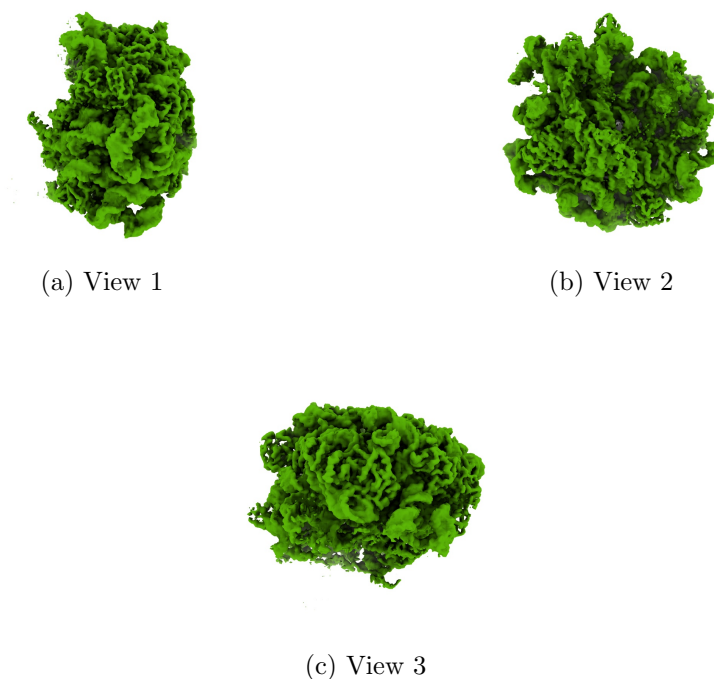
Figure 4: Isosurface at threshold=0.009160. Views generated by ChimeraX at a the following X, Y, Z angles: View 1 (0, -90, -90), View 2 (-90, 0, -90), View 3 (0, 0, 0).
