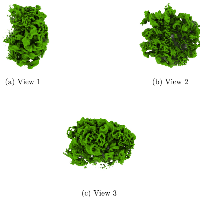
Figure 4: Isosurface at threshold=0.007290. Views generated by ChimeraX at a the following X, Y, Z angles: View 1 (0, -90, -90), View 2 (-90, 0, -90), View 3 (0, 0, 0).
