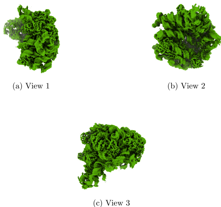
Figure 4: Isosurface at threshold=0.010400. Views generated by ChimeraX at a the following X, Y, Z angles: View 1 (0, -90, -90), View 2 (-90, 0, -90), View 3 (0, 0, 0).
