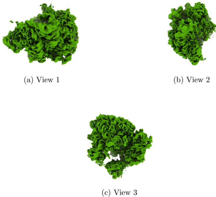
Figure 4: Isosurface at threshold=0.013200. Views generated by ChimeraX at a the following X, Y, Z angles: View 1 (0, -90, -90), View 2 (-90, 0, -90), View 3 (0, 0, 0).
