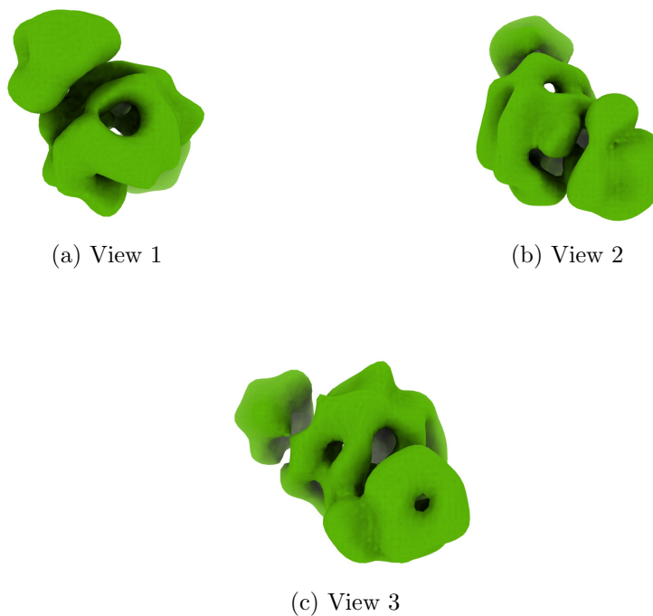
Figure 4: Isosurface at threshold=5.150000. Views generated by ChimeraX at a the following X, Y, Z angles: View 1 (0, -90, -90), View 2 (-90, 0, -90), View 3 (0, 0, 0).
