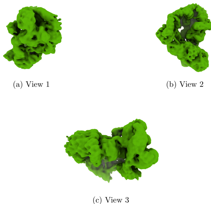
Figure 4: Isosurface at threshold=0.013500. Views generated by ChimeraX at a the following X, Y, Z angles: View 1 (0, -90, -90), View 2 (-90, 0, -90), View 3 (0, 0, 0).
