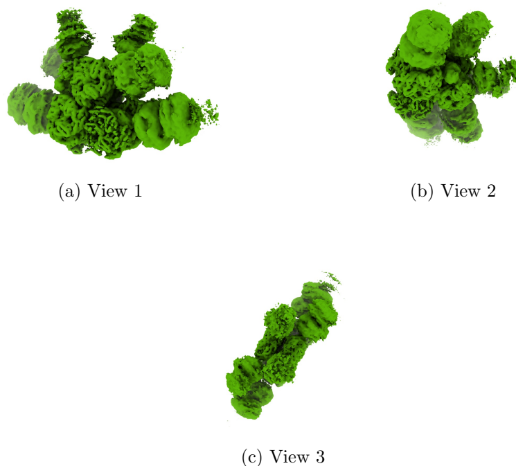
Figure 4: Isosurface at threshold=0.384000. Views generated by ChimeraX at a the following X, Y, Z angles: View 1 (0, -90, -90), View 2 (-90, 0, -90), View 3 (0, 0, 0).
