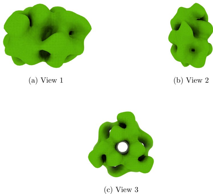
Figure 4: Isosurface at threshold=2.350000. Views generated by ChimeraX at a the following X, Y, Z angles: View 1 (0, -90, -90), View 2 (-90, 0, -90), View 3 (0, 0, 0).
