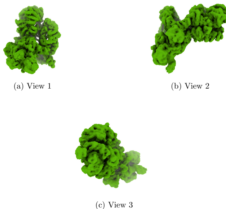
Figure 4: Isosurface at threshold=0.007800. Views generated by ChimeraX at a the following X, Y, Z angles: View 1 (0, -90, -90), View 2 (-90, 0, -90), View 3 (0, 0, 0).
