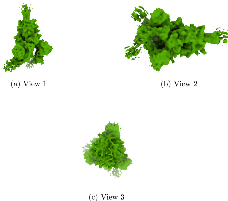
Figure 4: Isosurface at threshold=0.060000. Views generated by ChimeraX at a the following X, Y, Z angles: View 1 (0, -90, -90), View 2 (-90, 0, -90), View 3 (0, 0, 0).
