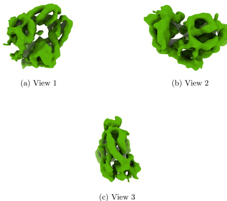
Figure 4: Isosurface at threshold=0.008450. Views generated by ChimeraX at a the following X, Y, Z angles: View 1 (0, -90, -90), View 2 (-90, 0, -90), View 3 (0, 0, 0).
