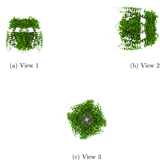
Figure 4: Isosurface at threshold=0.045000. Views generated by ChimeraX at a the following X, Y, Z angles: View 1 (0, -90, -90), View 2 (-90, 0, -90), View 3 (0, 0, 0).
