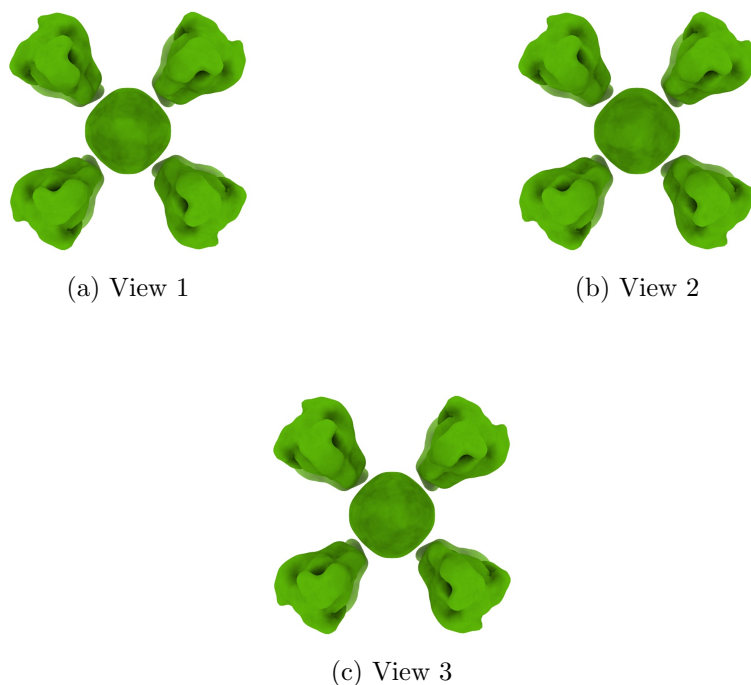
Figure 4: Isosurface at threshold=0.002660. Views generated by ChimeraX at a the following X, Y, Z angles: View 1 (0, -90, -90), View 2 (-90, 0, -90), View 3 (0, 0, 0).
