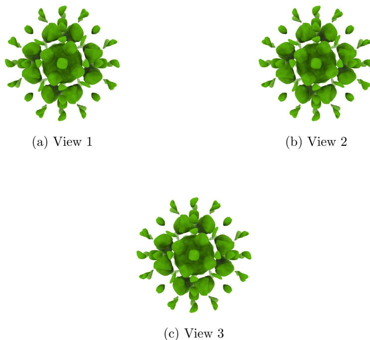
Figure 4: Isosurface at threshold=0.005390. Views generated by ChimeraX at a the following X, Y, Z angles: View 1 (0, -90, -90), View 2 (-90, 0, -90), View 3 (0, 0, 0).
