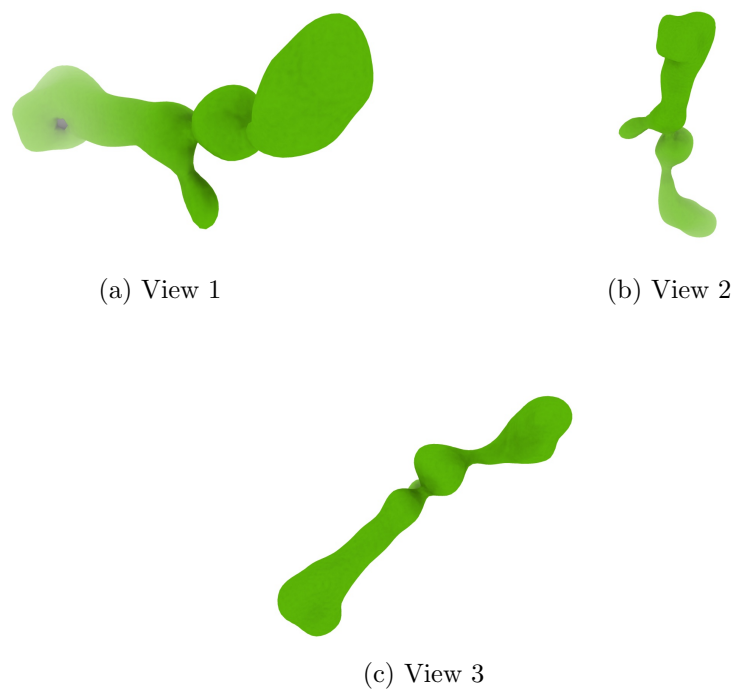
Figure 4: Isosurface at threshold=9.840000. Views generated by ChimeraX at a the following X, Y, Z angles: View 1 (0, -90, -90), View 2 (-90, 0, -90), View 3 (0, 0, 0).
