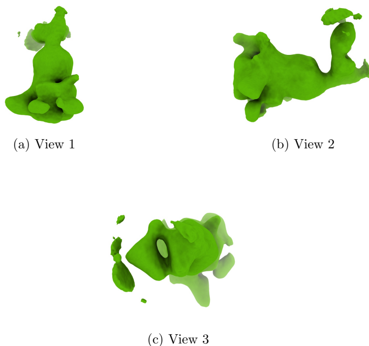
Figure 4: Isosurface at threshold=0.005960. Views generated by ChimeraX at a the following X, Y, Z angles: View 1 (0, -90, -90), View 2 (-90, 0, -90), View 3 (0, 0, 0).
