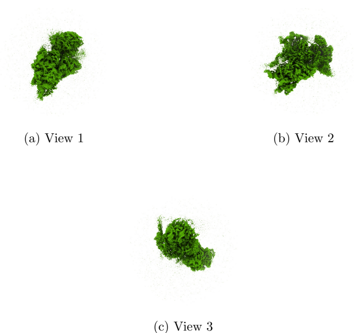
Figure 4: Isosurface at threshold=0.051100. Views generated by ChimeraX at a the following X, Y, Z angles: View 1 (0, -90, -90), View 2 (-90, 0, -90), View 3 (0, 0, 0).
