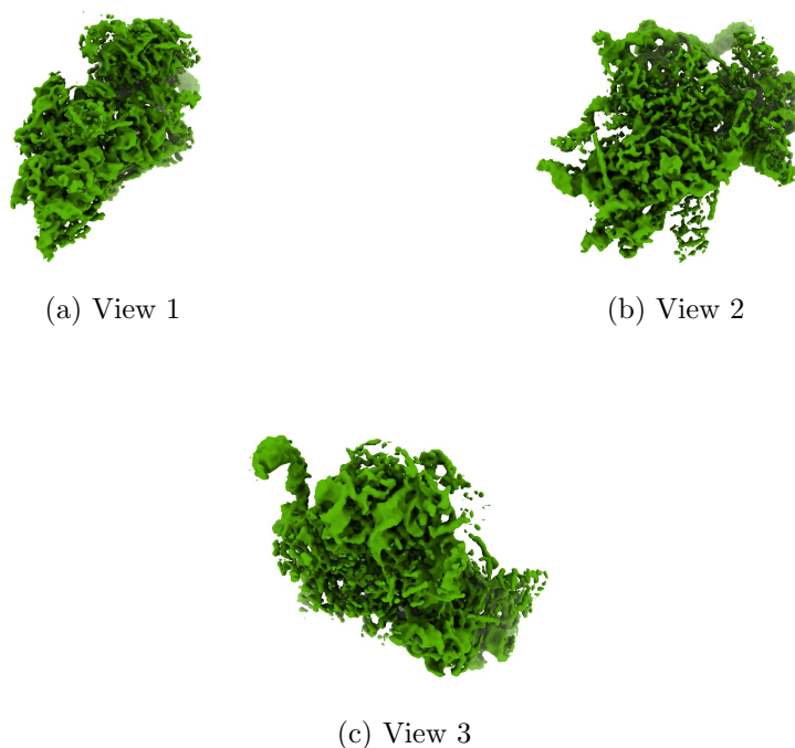
Figure 4: Isosurface at threshold=0.010700. Views generated by ChimeraX at a the following X, Y, Z angles: View 1 (0, -90, -90), View 2 (-90, 0, -90), View 3 (0, 0, 0).
