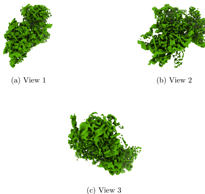
Figure 4: Isosurface at threshold=0.009910. Views generated by ChimeraX at a the following X, Y, Z angles: View 1 (0, -90, -90), View 2 (-90, 0, -90), View 3 (0, 0, 0).
