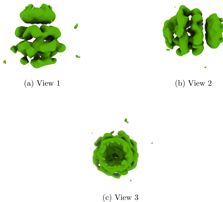
Figure 4: Isosurface at threshold=0.314000. Views generated by ChimeraX at a the following X, Y, Z angles: View 1 (0, -90, -90), View 2 (-90, 0, -90), View 3 (0, 0, 0).
