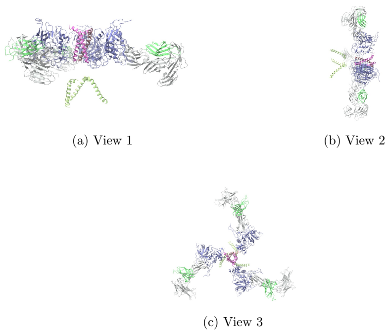
Figure 10: Input atomic model Views generated by ChimeraX at a the following X, Y, Z angles: View 1 (0, -90, -90), View 2 (-90, 0, -90), View 3 (0, 0, 0).
