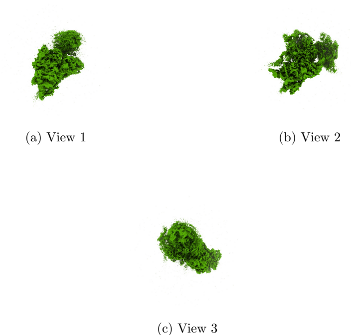
Figure 4: Isosurface at threshold=0.007750. Views generated by ChimeraX at a the following X, Y, Z angles: View 1 (0, -90, -90), View 2 (-90, 0, -90), View 3 (0, 0, 0).
