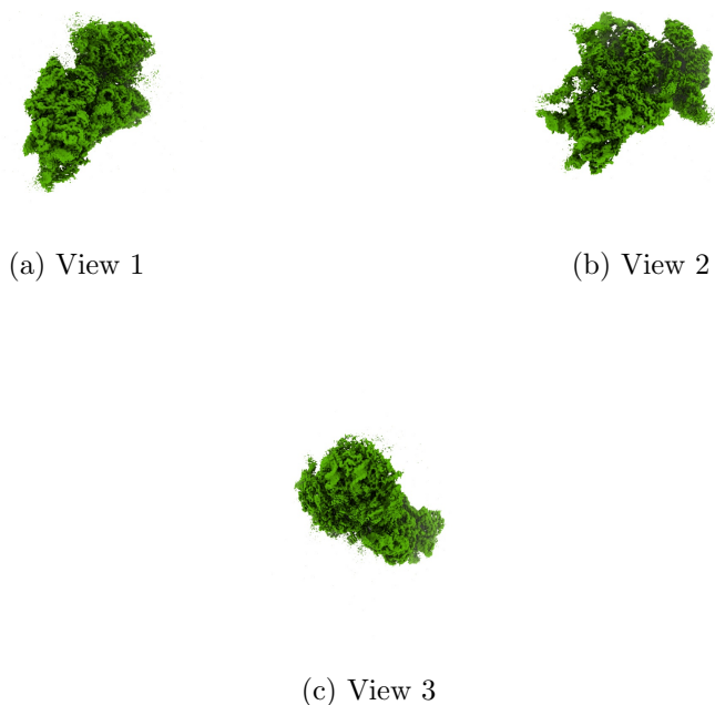
Figure 4: Isosurface at threshold=0.011500. Views generated by ChimeraX at a the following X, Y, Z angles: View 1 (0, -90, -90), View 2 (-90, 0, -90), View 3 (0, 0, 0).
