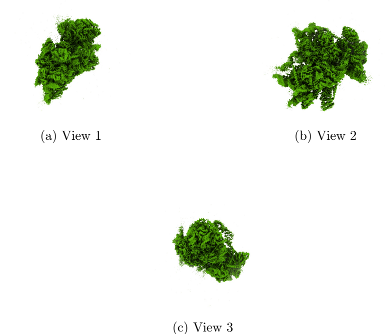
Figure 4: Isosurface at threshold=0.011400. Views generated by ChimeraX at a the following X, Y, Z angles: View 1 (0, -90, -90), View 2 (-90, 0, -90), View 3 (0, 0, 0).
