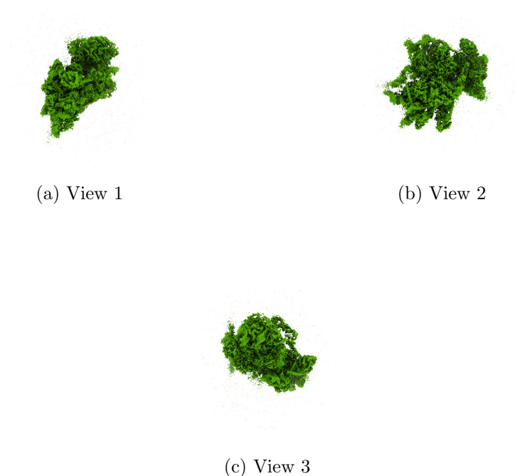
Figure 4: Isosurface at threshold=0.013100. Views generated by ChimeraX at a the following X, Y, Z angles: View 1 (0, -90, -90), View 2 (-90, 0, -90), View 3 (0, 0, 0).
