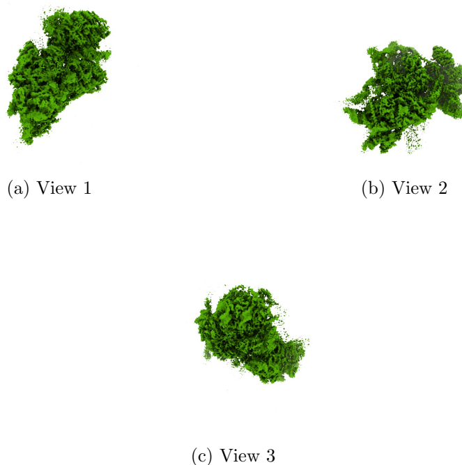
Figure 4: Isosurface at threshold=0.009880. Views generated by ChimeraX at a the following X, Y, Z angles: View 1 (0, -90, -90), View 2 (-90, 0, -90), View 3 (0, 0, 0).
